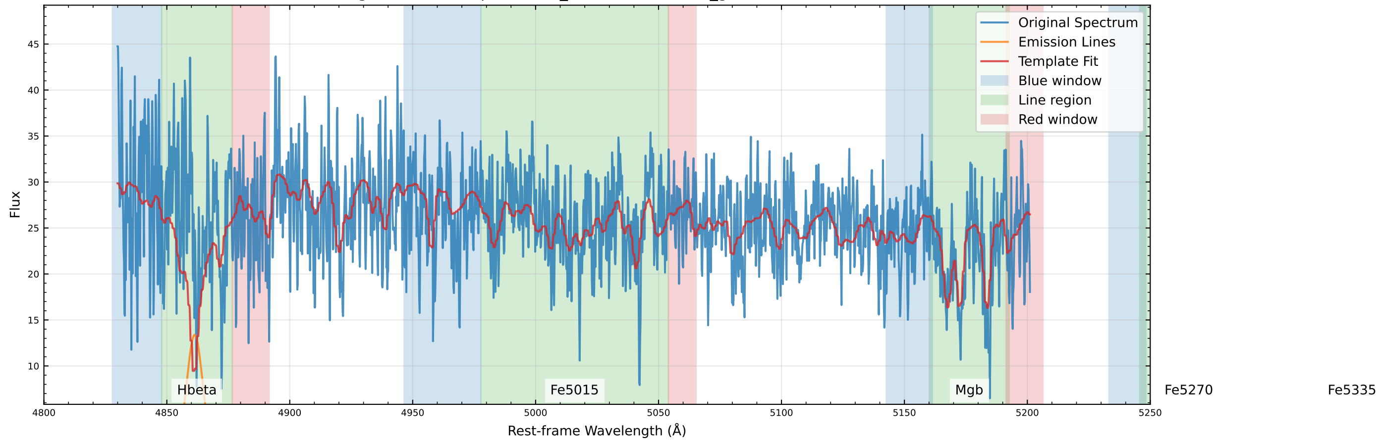
Original Data Comparison (v_star=36.4 km/s, v_gas=-126.7 km/s)
