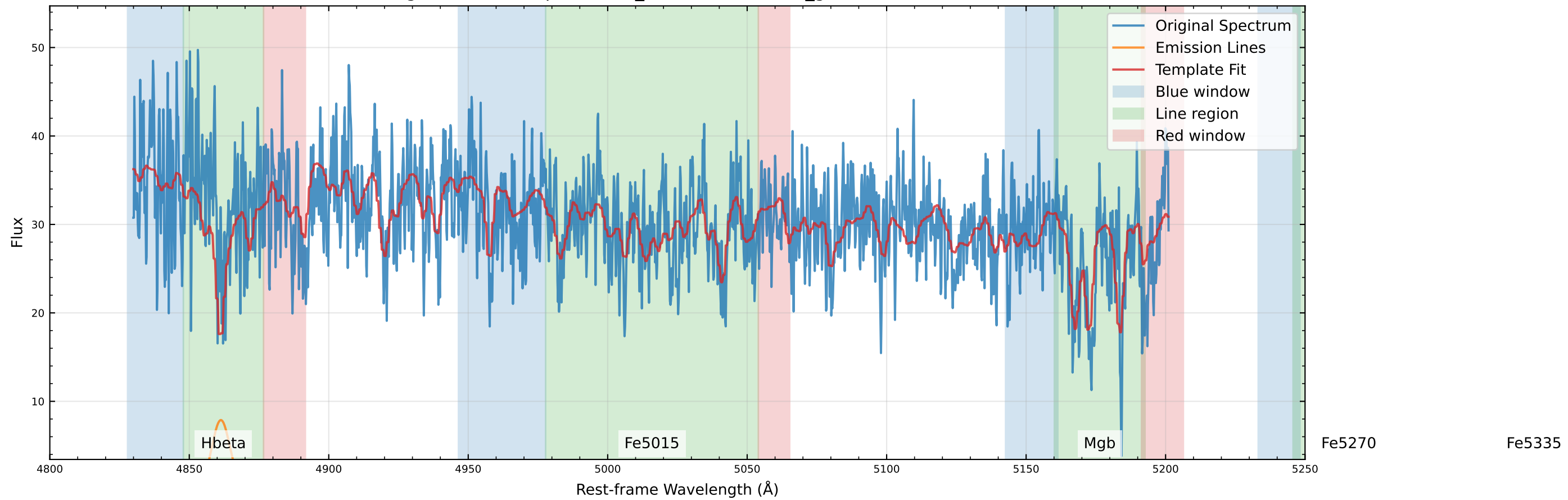
Original Data Comparison (v_star=29.0 km/s, v_gas=-172.8 km/s)
