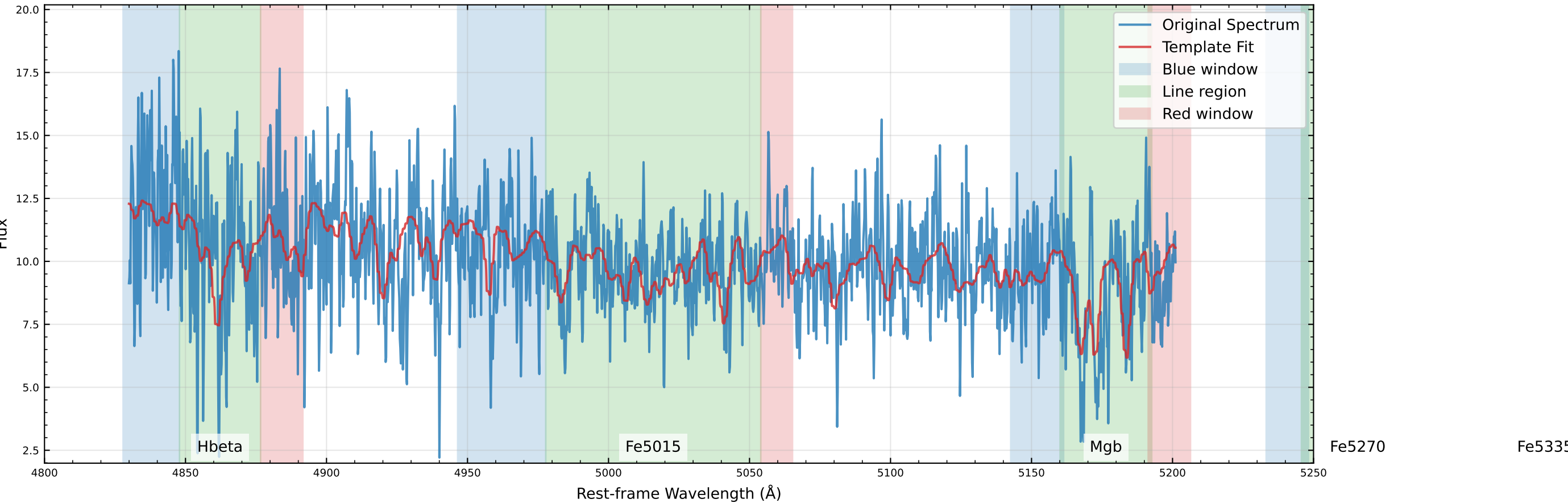
Original Data Comparison (v_star=61.0 km/s)
