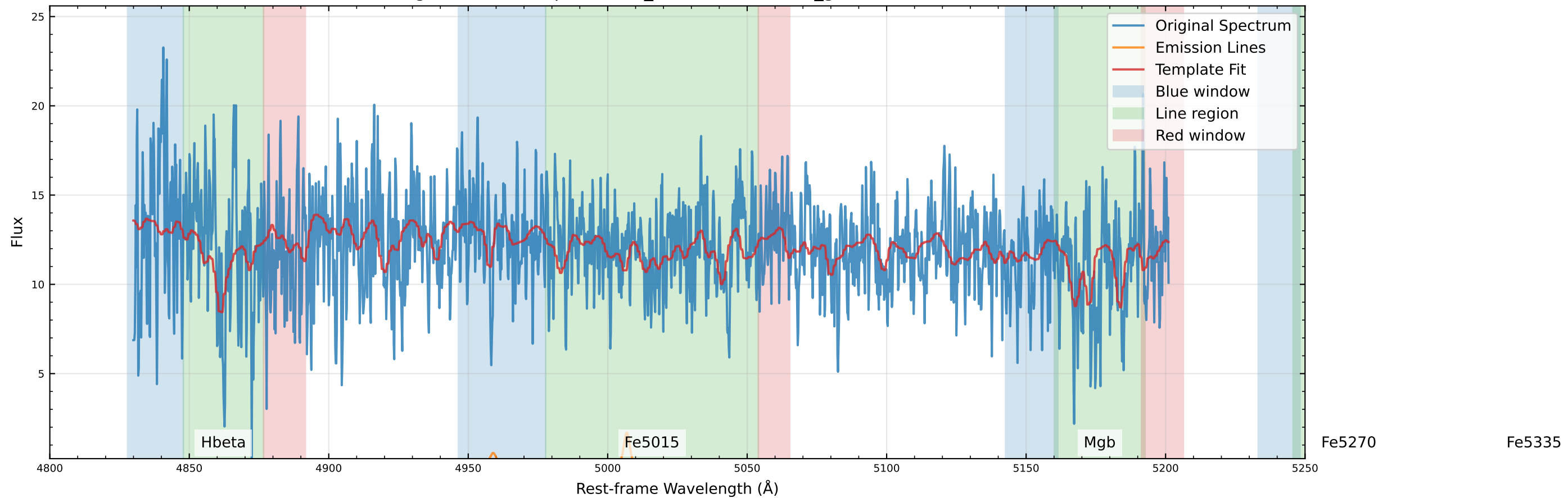
Original Data Comparison (v_star=97.7 km/s, v_gas=68.8 km/s)
