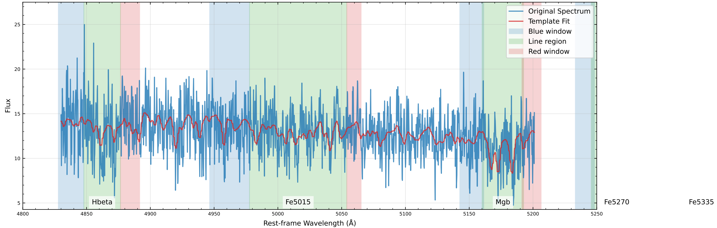
Original Data Comparison (v_star=44.6 km/s)
