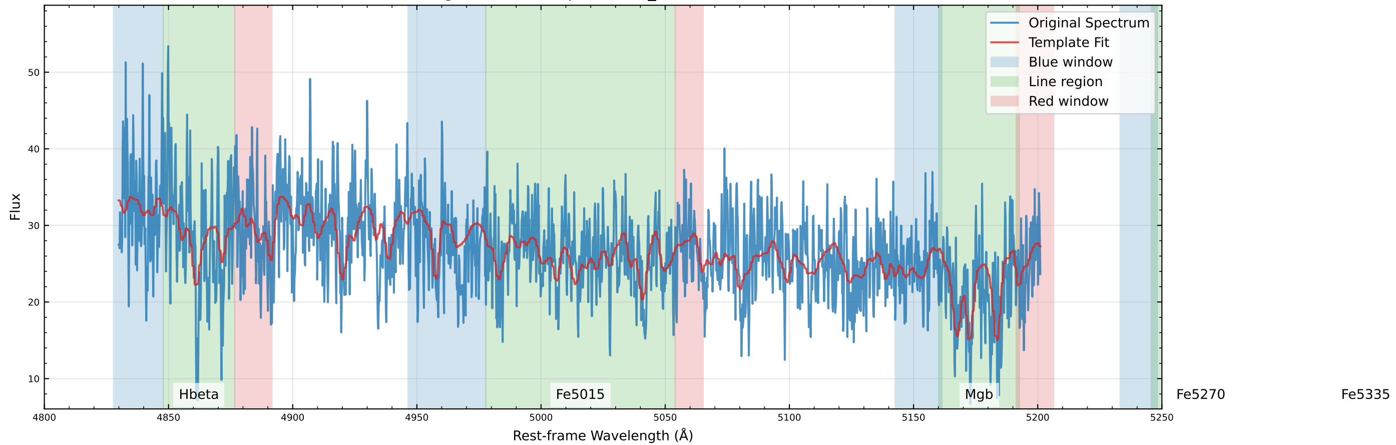
Original Data Comparison (v_star=23.4 km/s)
