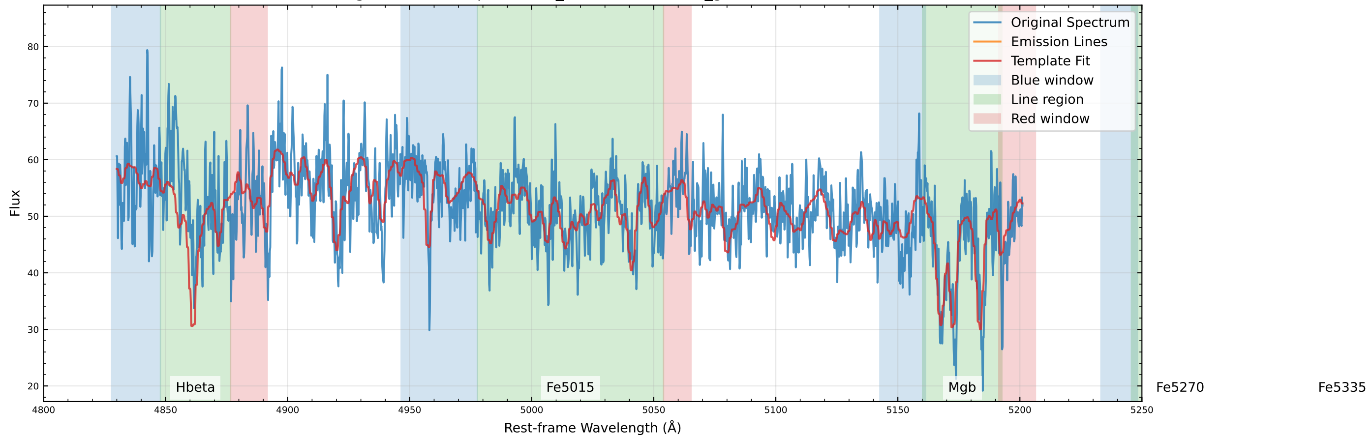
Original Data Comparison (v_star=36.1 km/s, v_gas=-263.9 km/s)
