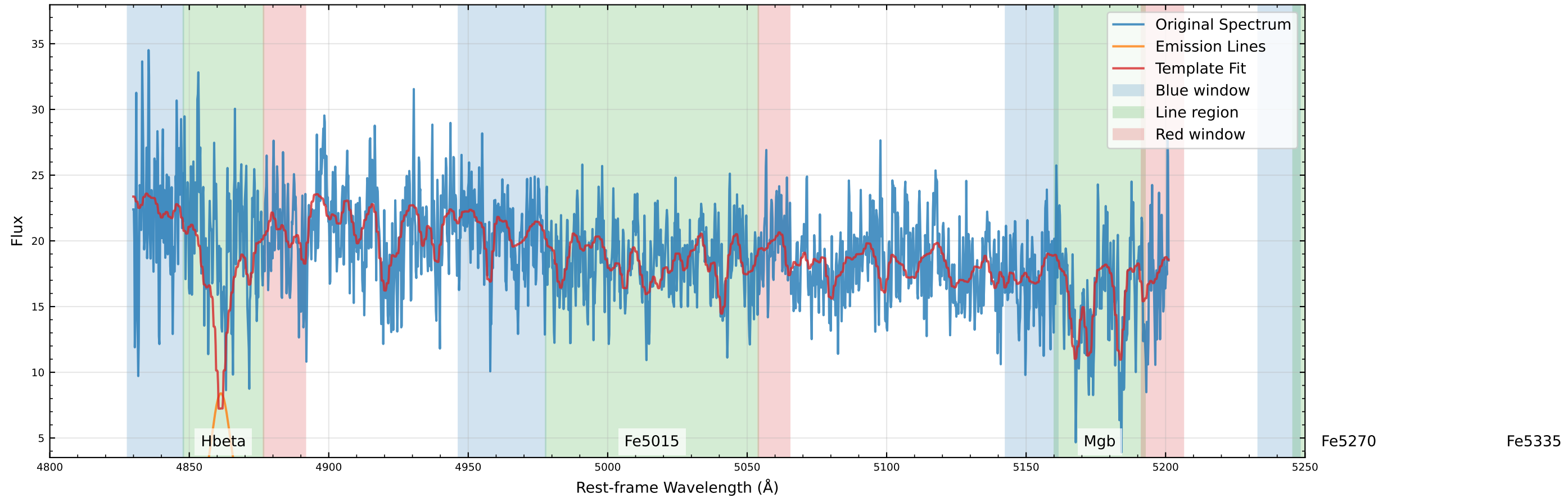
Original Data Comparison (v_star=41.0 km/s, v_gas=20.6 km/s)
