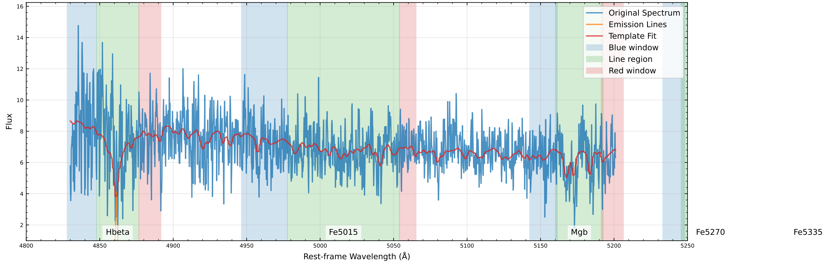
Original Data Comparison (v_star=49.7 km/s, v_gas=141.9 km/s)
