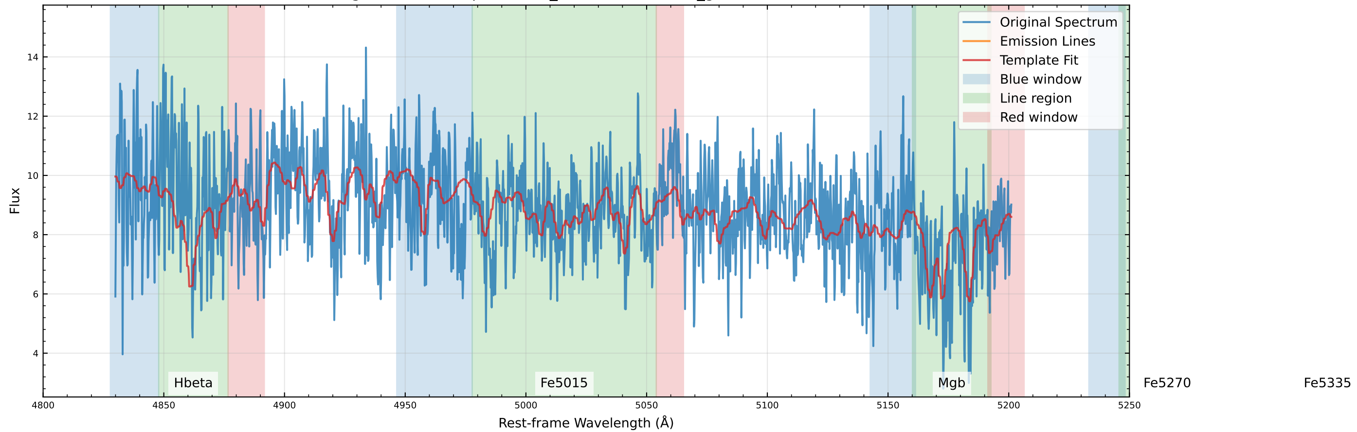
Original Data Comparison (v_star=40.4 km/s, v_gas=-202.7 km/s)
