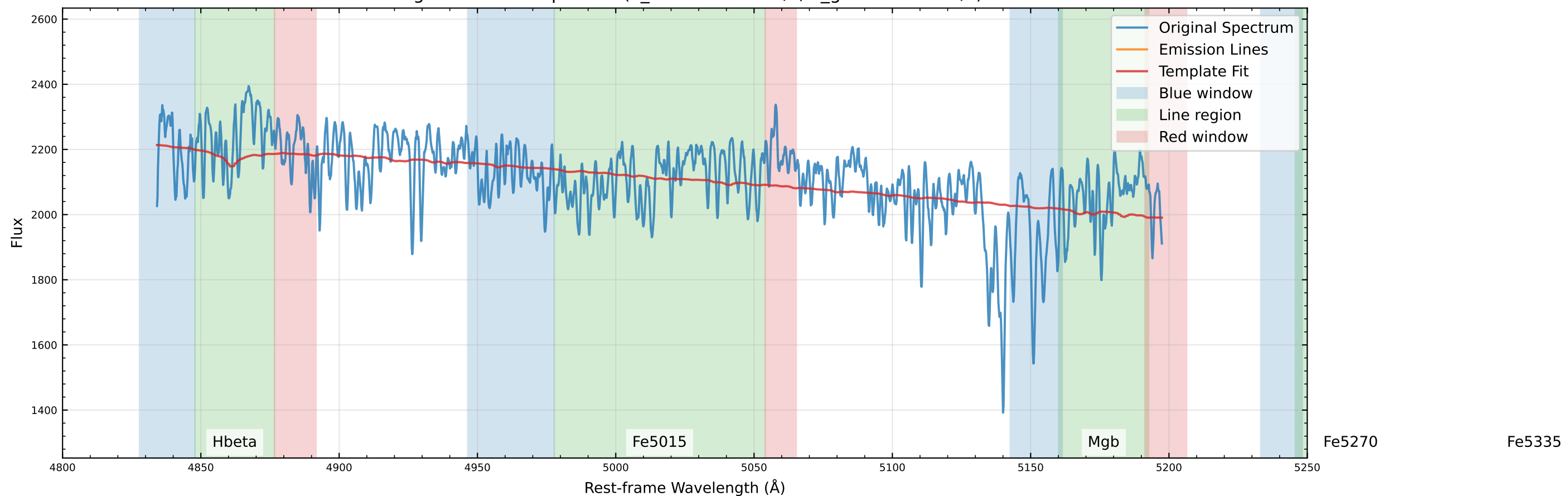
Original Data Comparison (v_star=126.1 km/s, v_gas=426.1 km/s)
