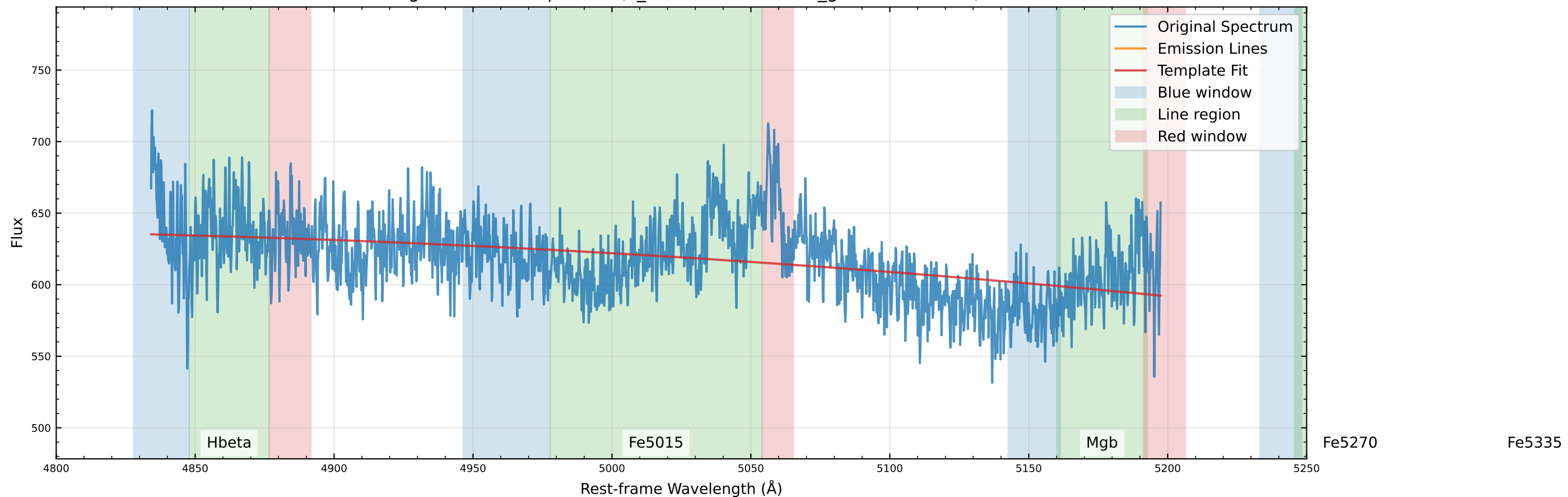
Original Data Comparison (v_star=166.2 km/s, v_gas=344.6 km/s)
