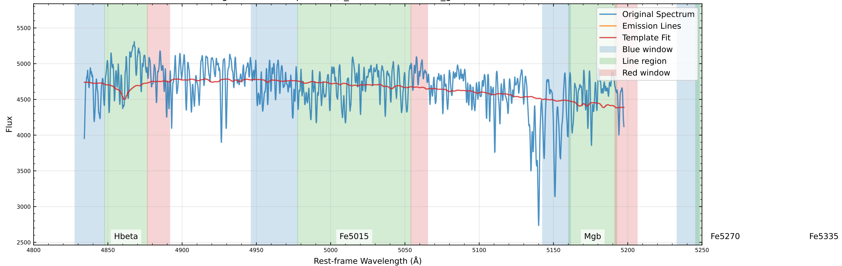
Original Data Comparison (v_star=101.6 km/s, v_gas=401.6 km/s)
