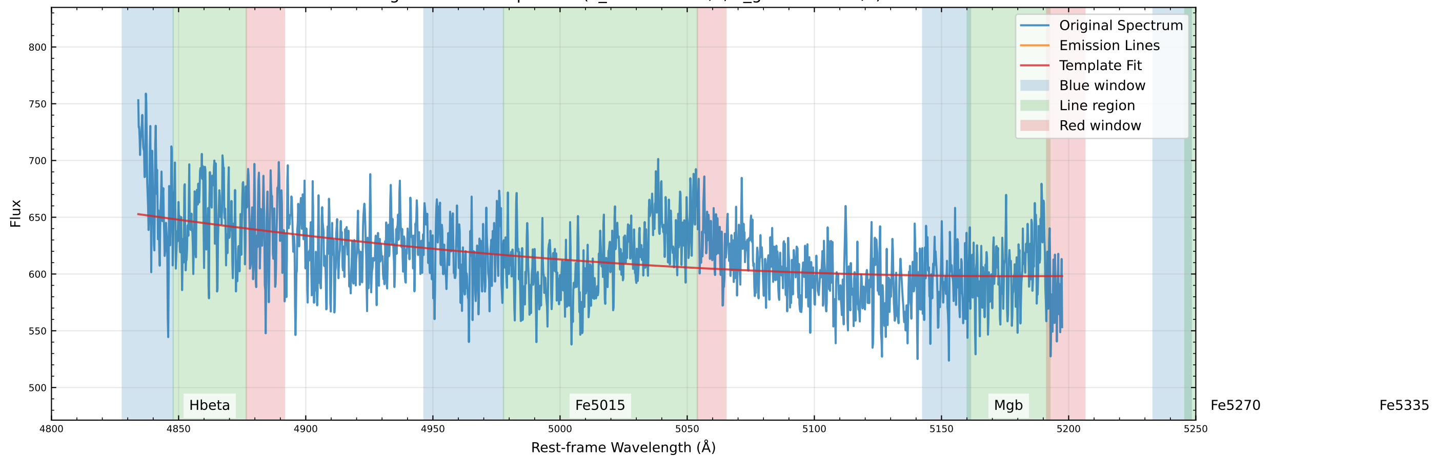
Original Data Comparison (v_star=0.0 km/s, v_gas=22.1 km/s)
