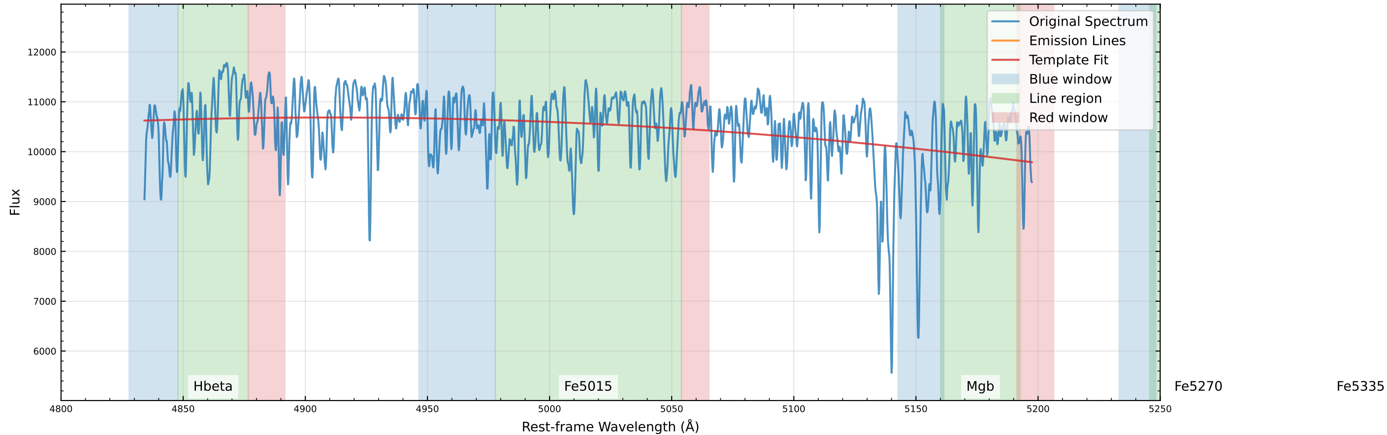
Original Data Comparison (v_star=87.8 km/s, v_gas=67.9 km/s)
