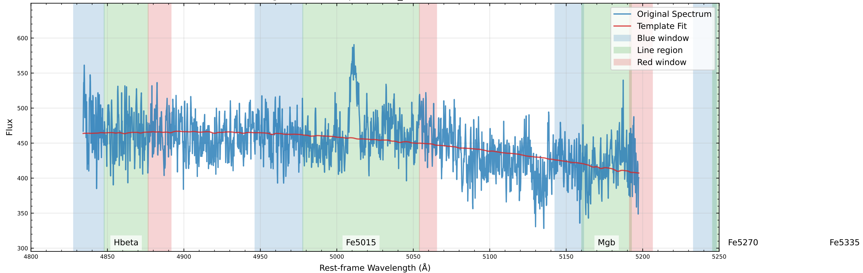
Original Data Comparison (v_star=-116.0 km/s)
