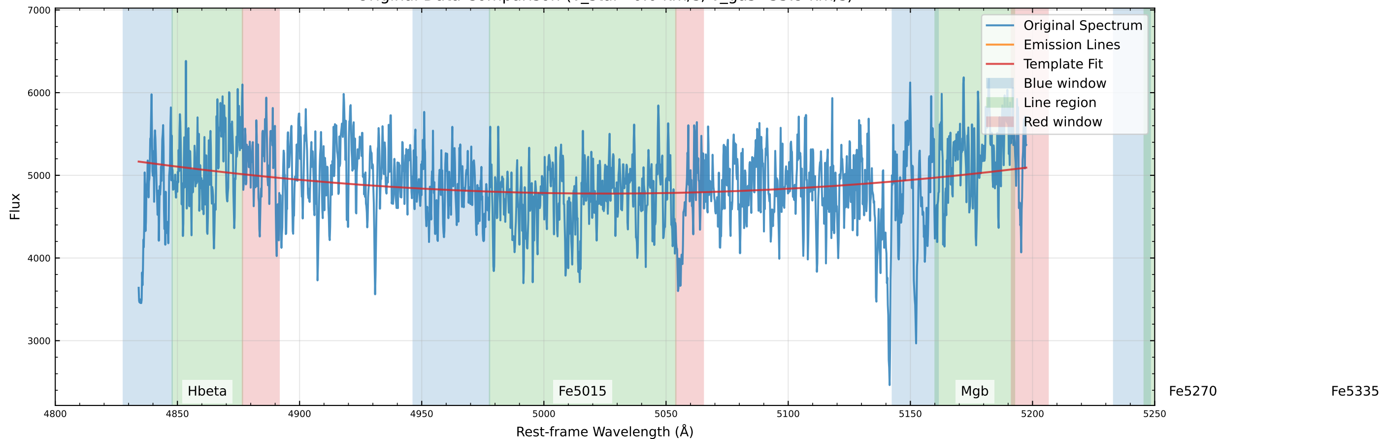
Original Data Comparison (v_star=0.0 km/s, v_gas=35.9 km/s)
