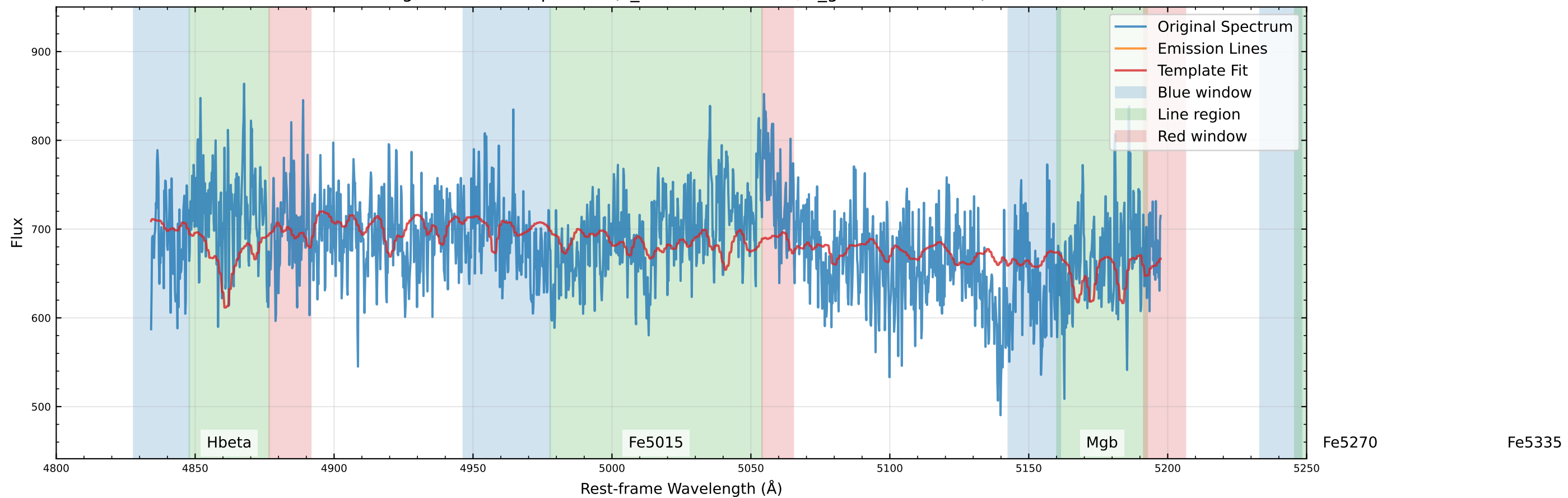
Original Data Comparison (v_star=-547.4 km/s, v_gas=-514.4 km/s)
