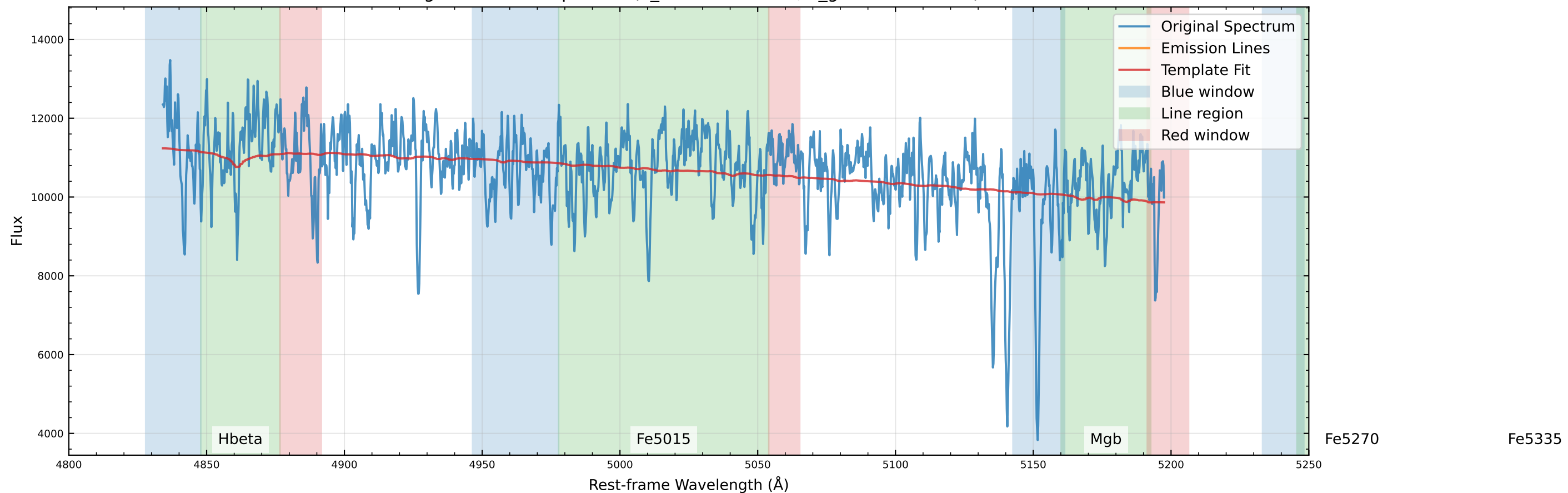
Original Data Comparison (v_star=84.5 km/s, v_gas=356.9 km/s)
