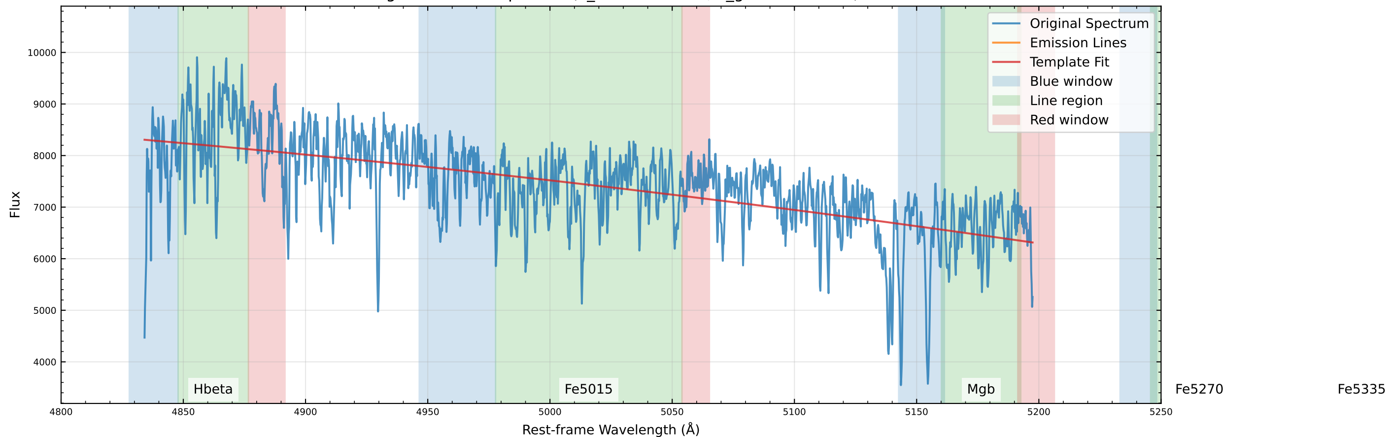
Original Data Comparison (v_star=0.0 km/s, v_gas=54.6 km/s)
