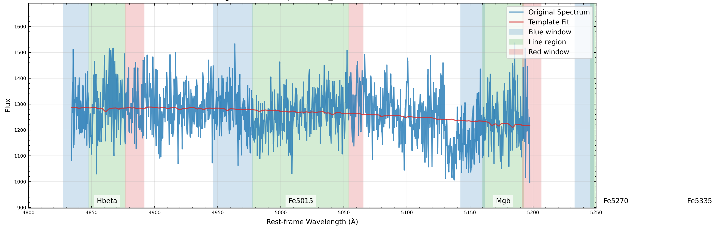
Original Data Comparison ( v_{\text{star}}=-1959.5 km/s)
