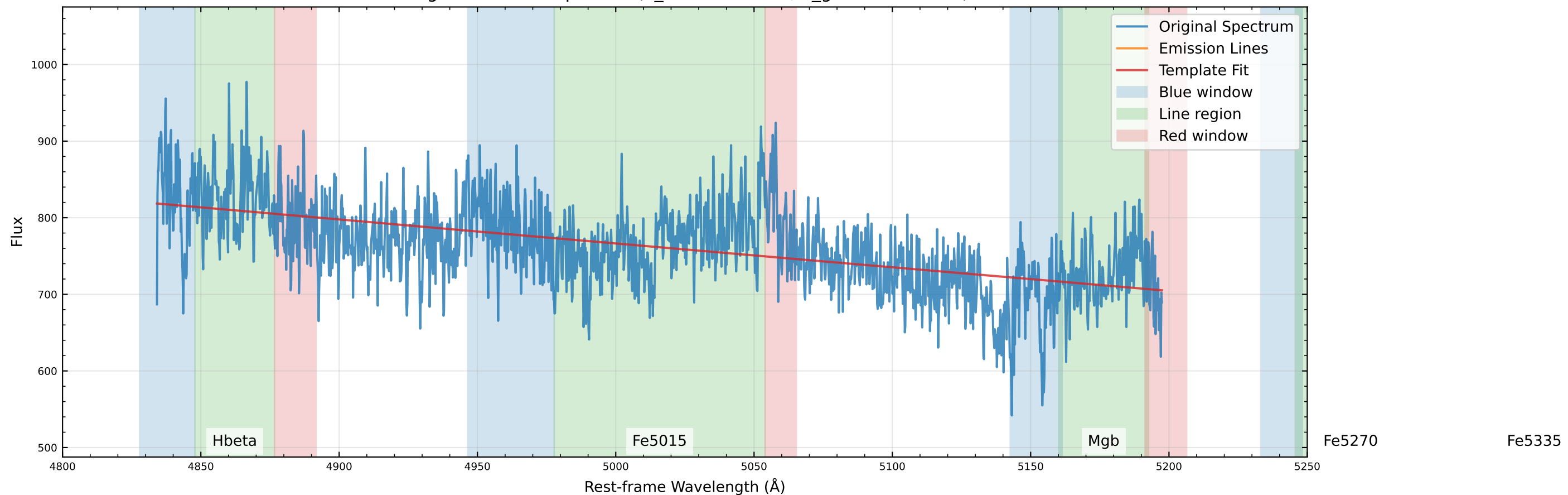
Original Data Comparison (v_star=0.0 km/s, v_gas=-39.1 km/s)
