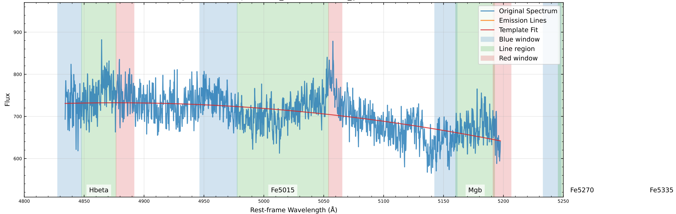
Original Data Comparison (v_star=0.0 km/s, v_gas=300.0 km/s)
