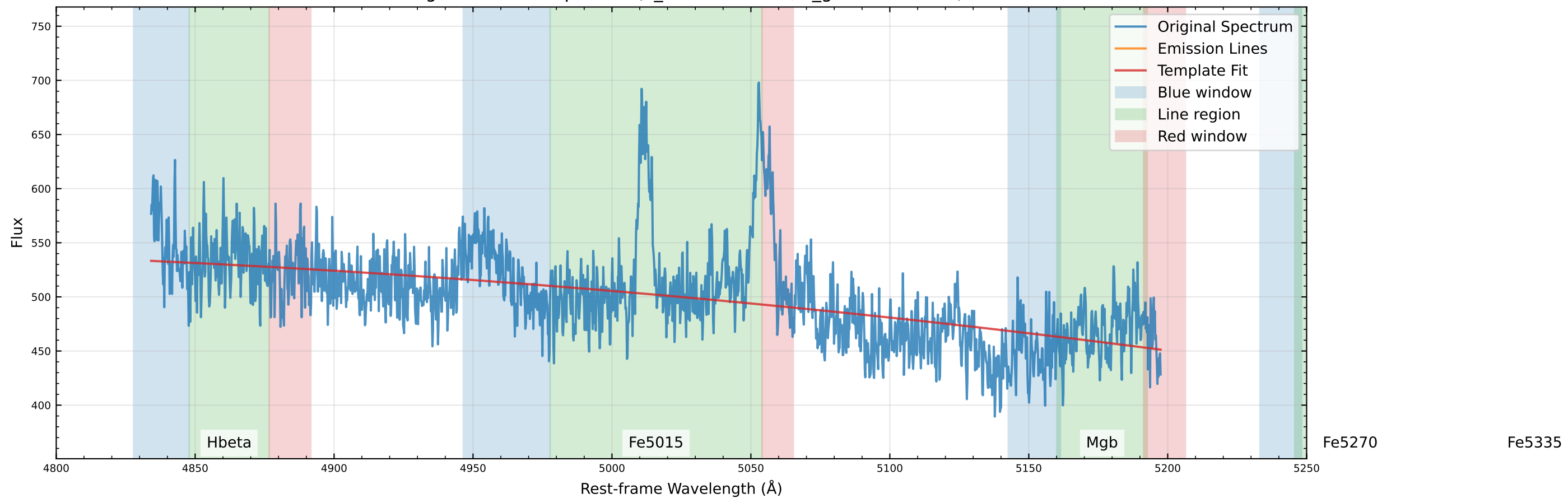
Original Data Comparison (v_star=0.0 km/s, v_gas=42.4 km/s)
