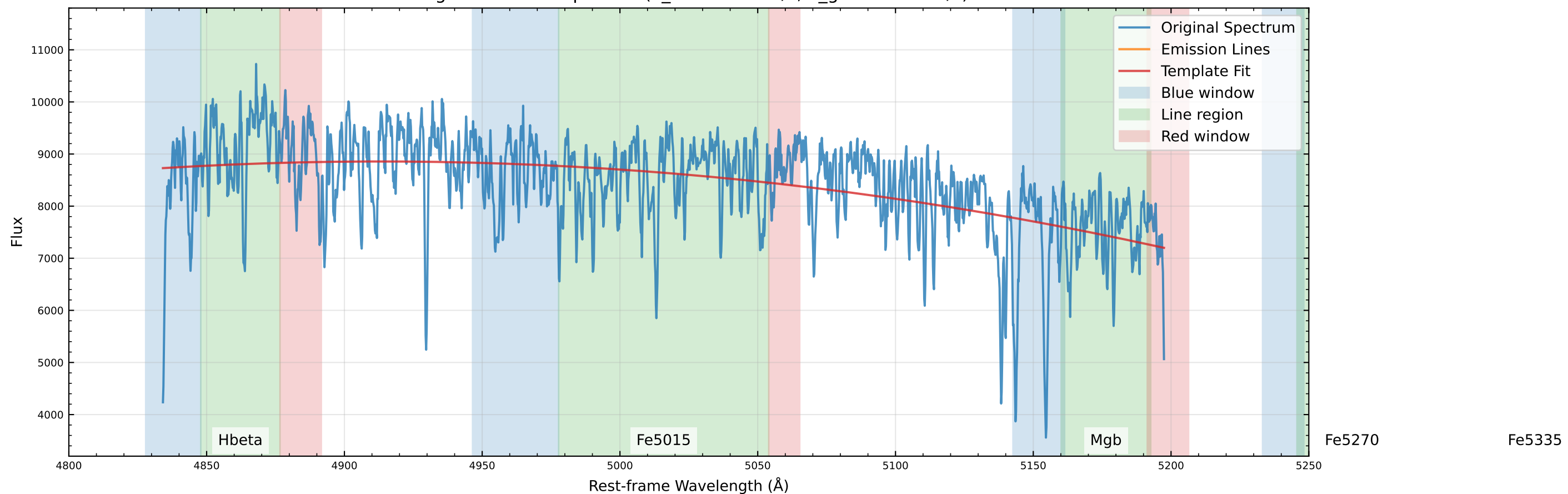
Original Data Comparison (v_star=0.0 km/s, v_gas=54.7 km/s)
