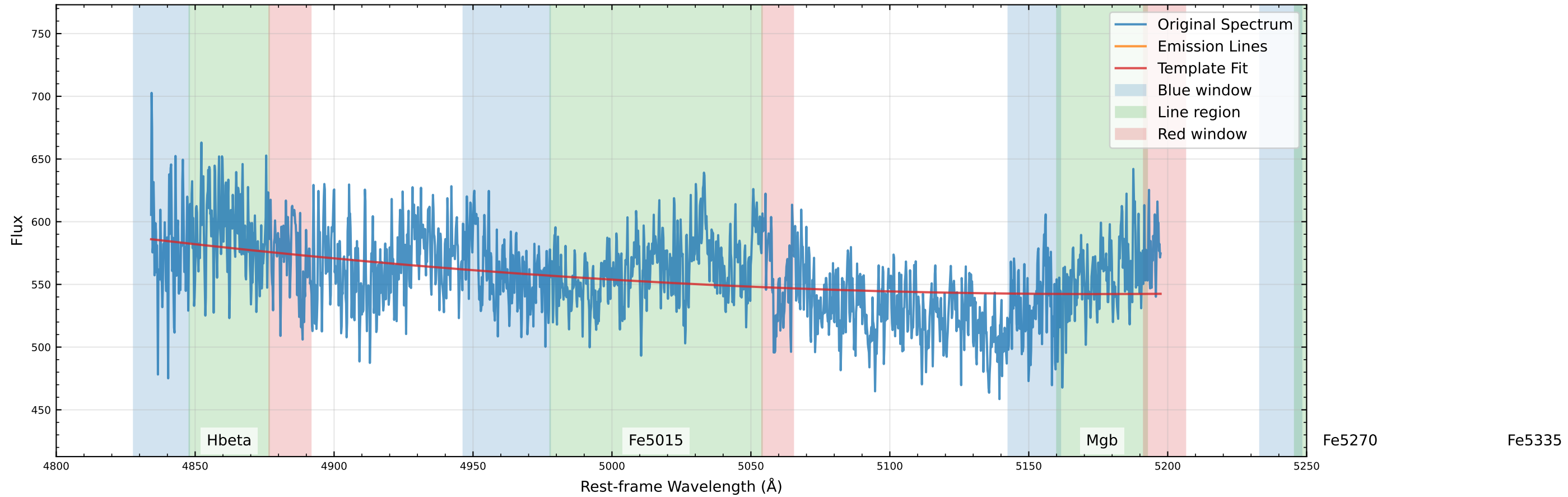
Original Data Comparison (v_star=0.0 km/s, v_gas=-43.0 km/s)
