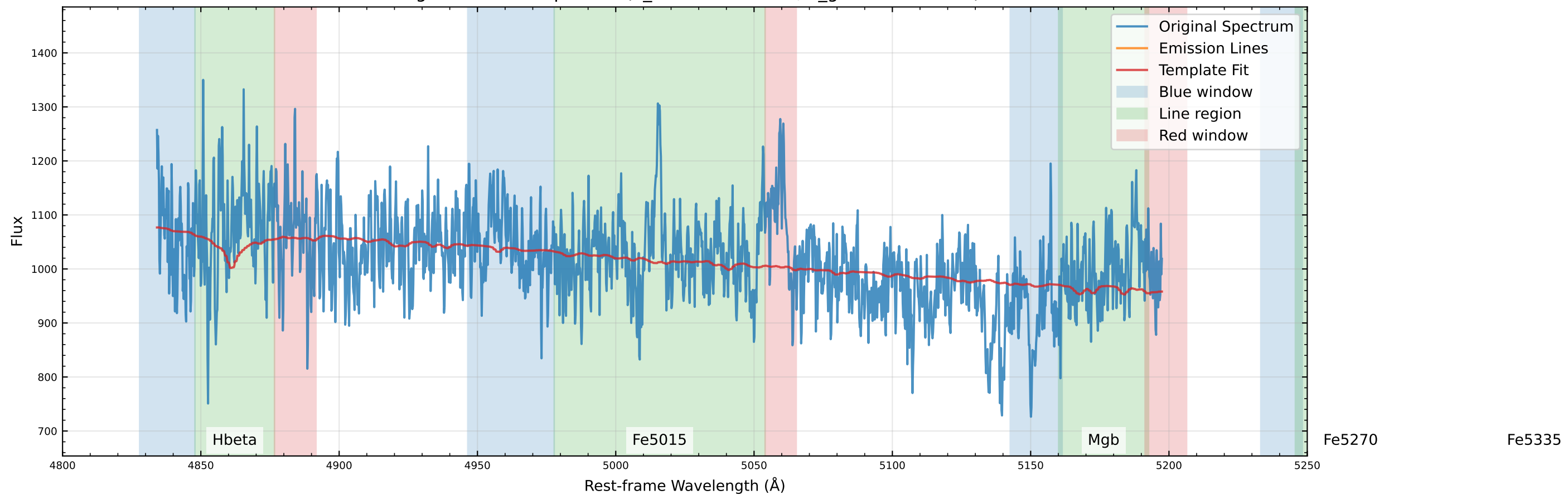
Original Data Comparison (v_star=-91.8 km/s, v_gas=208.2 km/s)
