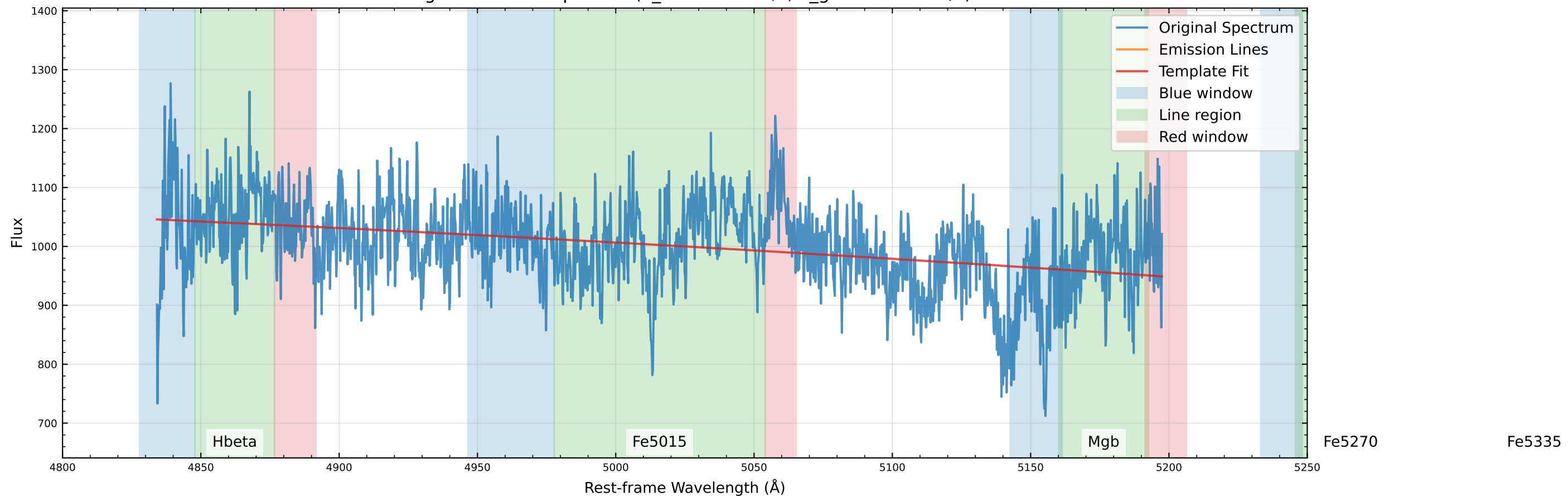
Original Data Comparison (v_star=0.0 km/s, v_gas=160.5 km/s)
