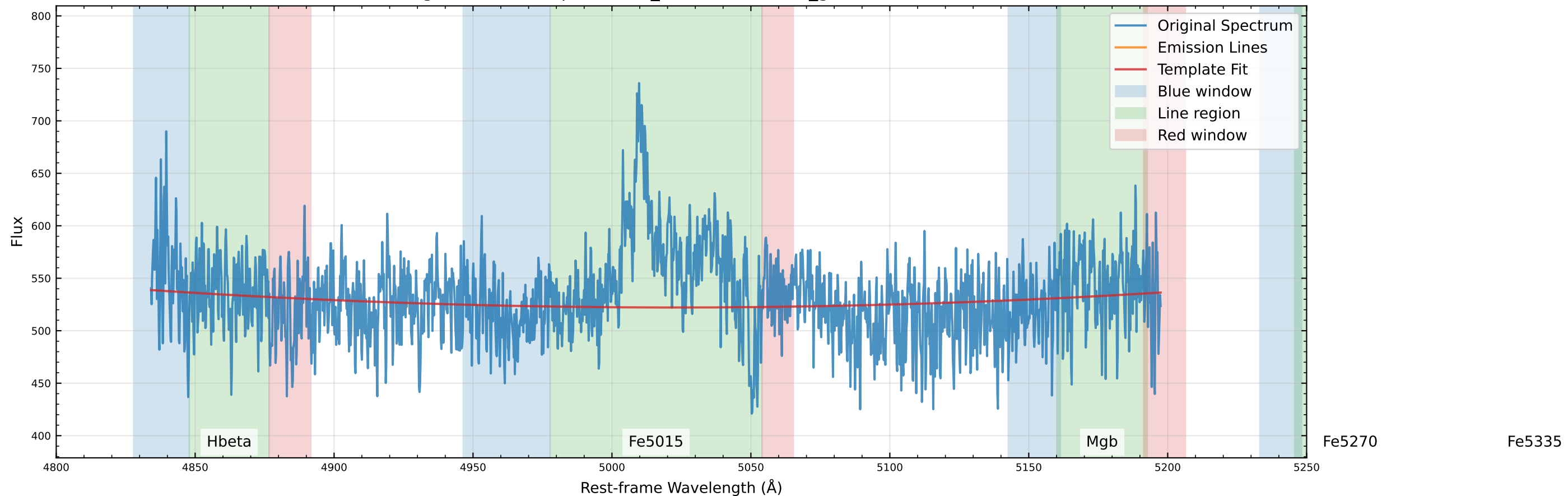
Original Data Comparison (v_star=0.0 km/s, v_gas=-14.2 km/s)
