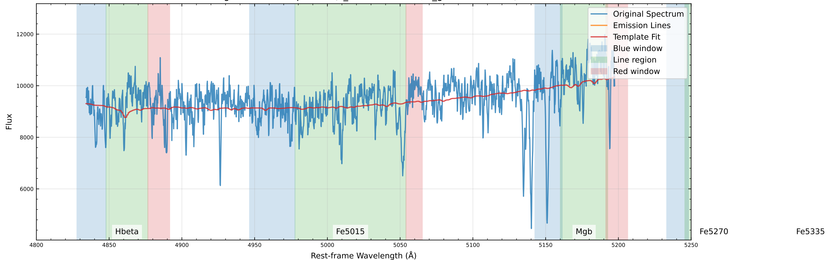
Original Data Comparison (v_star=55.9 km/s, v_gas=272.3 km/s)
