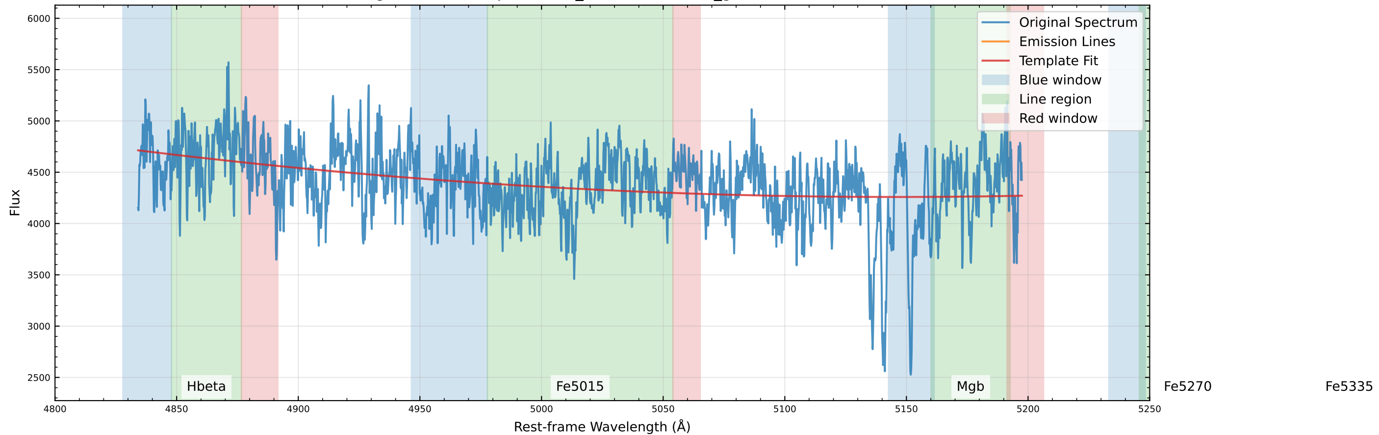
Original Data Comparison (v_star=0.0 km/s, v_gas=-17.3 km/s)
