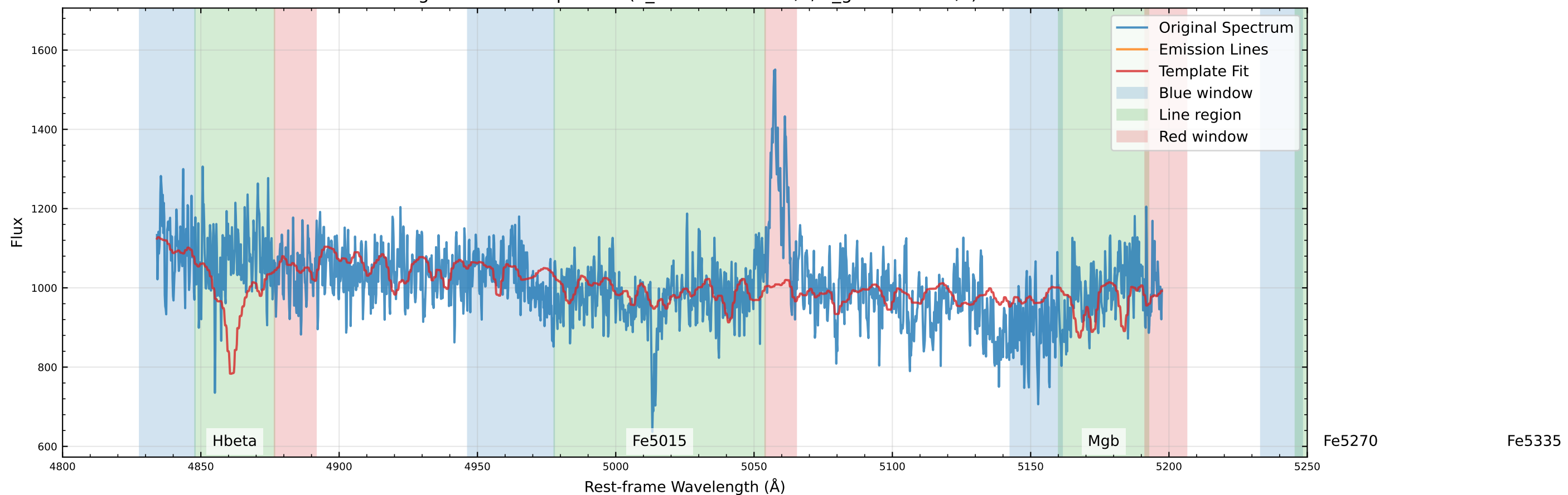
Original Data Comparison (v_star=-215.2 km/s, v_gas=-6.9 km/s)
