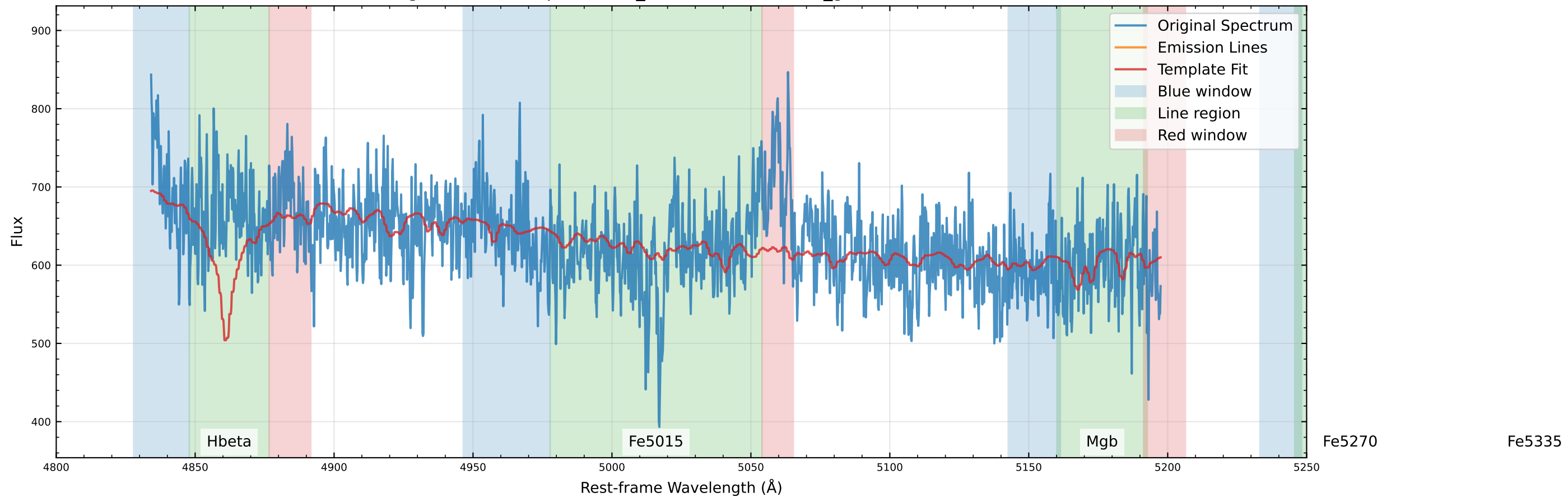
Original Data Comparison ( v_{\text{star}}=-387.9 km/s, v_{\text{gas}}=-87.9 km/s)
