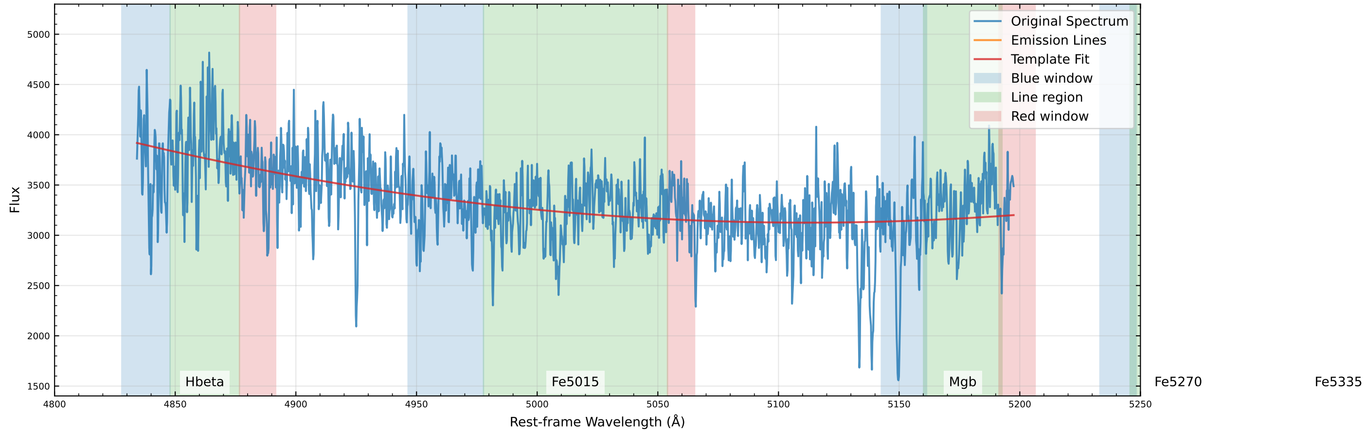
Original Data Comparison (v_star=-20.9 km/s, v_gas=-10.9 km/s)
