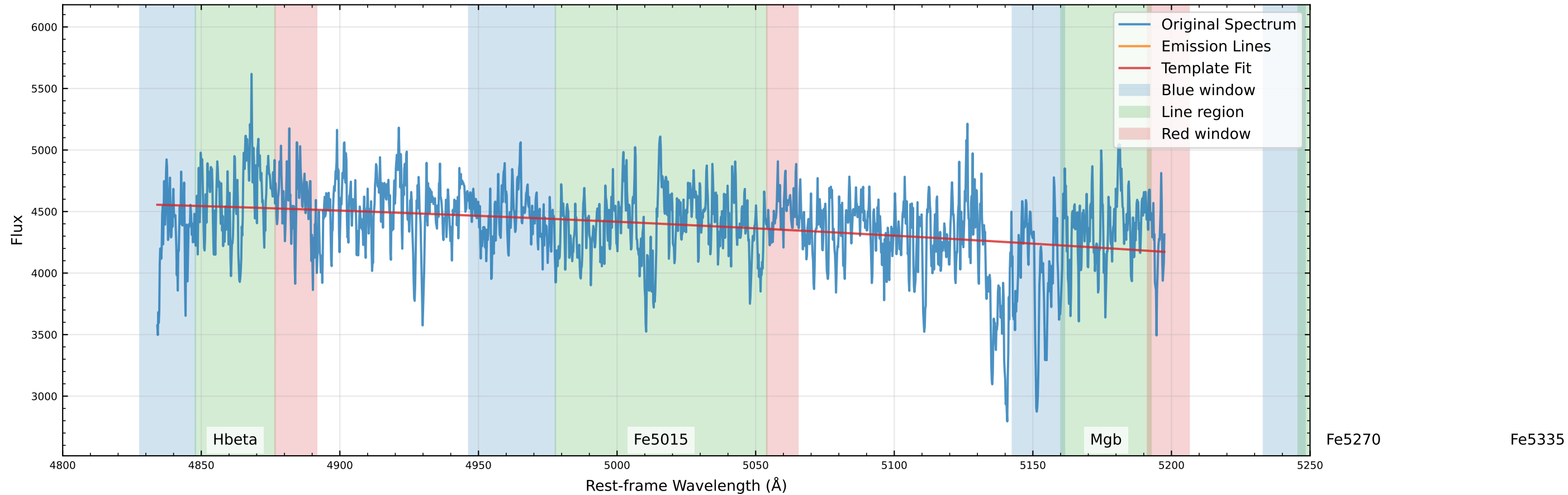
Original Data Comparison (v_star=0.0 km/s, v_gas=-25.9 km/s)
