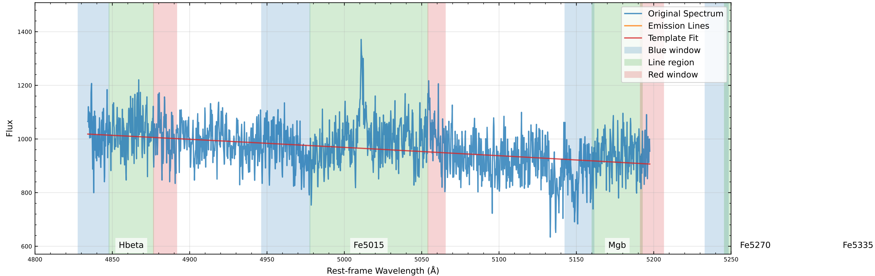
Original Data Comparison (v_star=0.0 km/s, v_gas=269.9 km/s)
