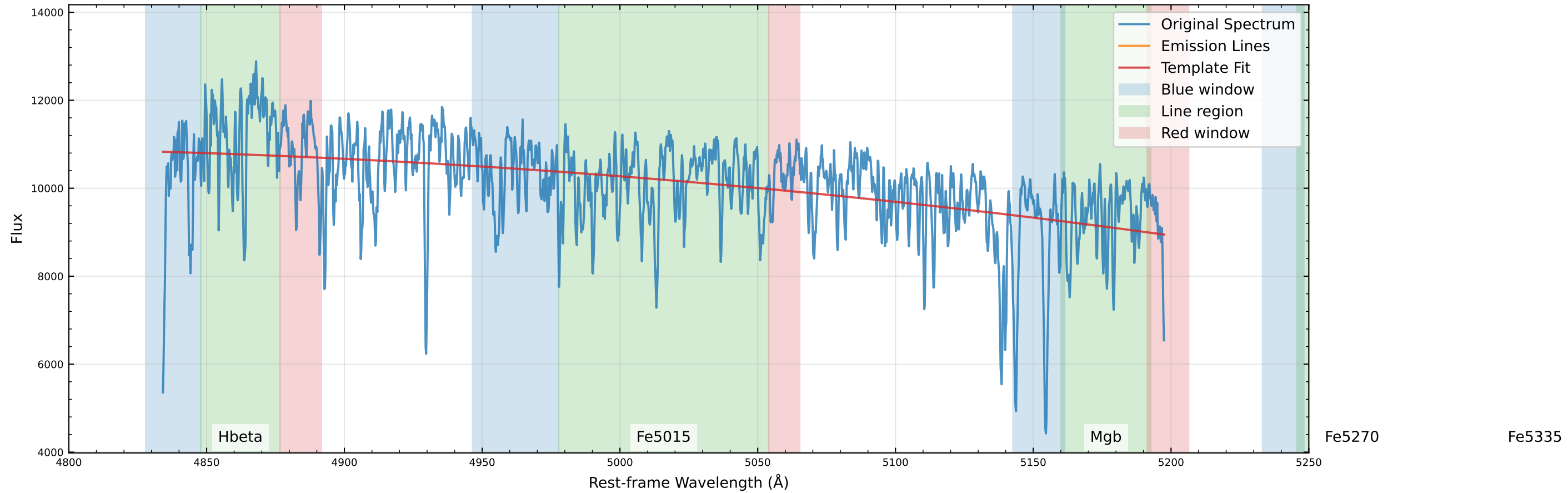
Original Data Comparison (v_star=0.0 km/s, v_gas=5.6 km/s)
