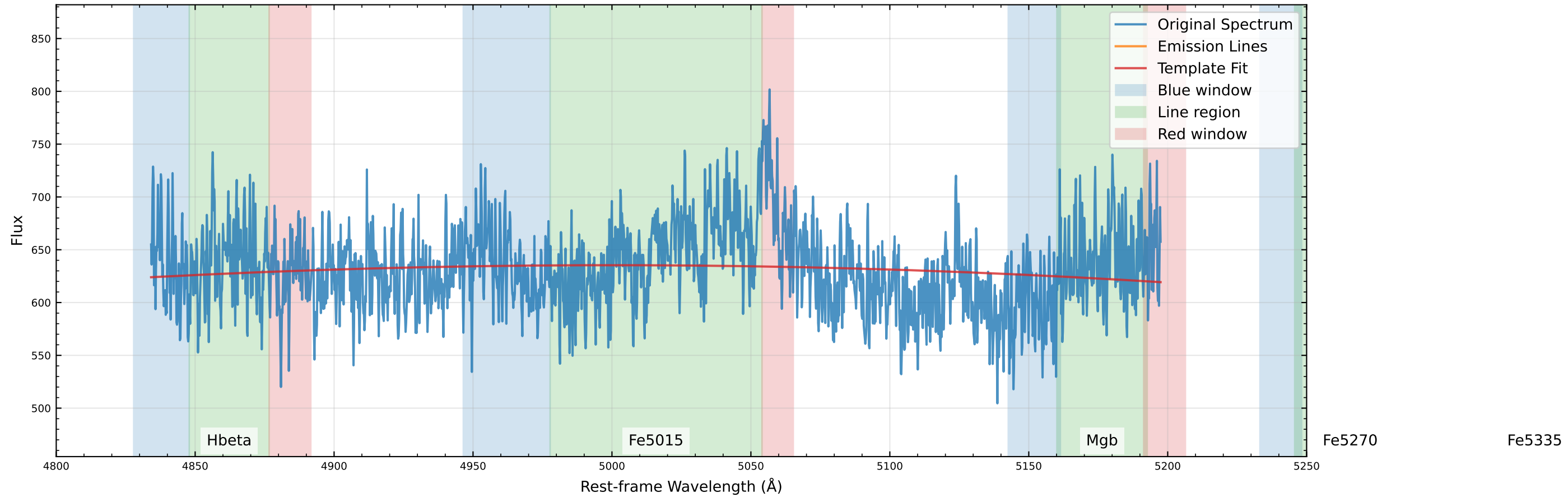
Original Data Comparison (v_star=0.0 km/s, v_gas=122.3 km/s)
