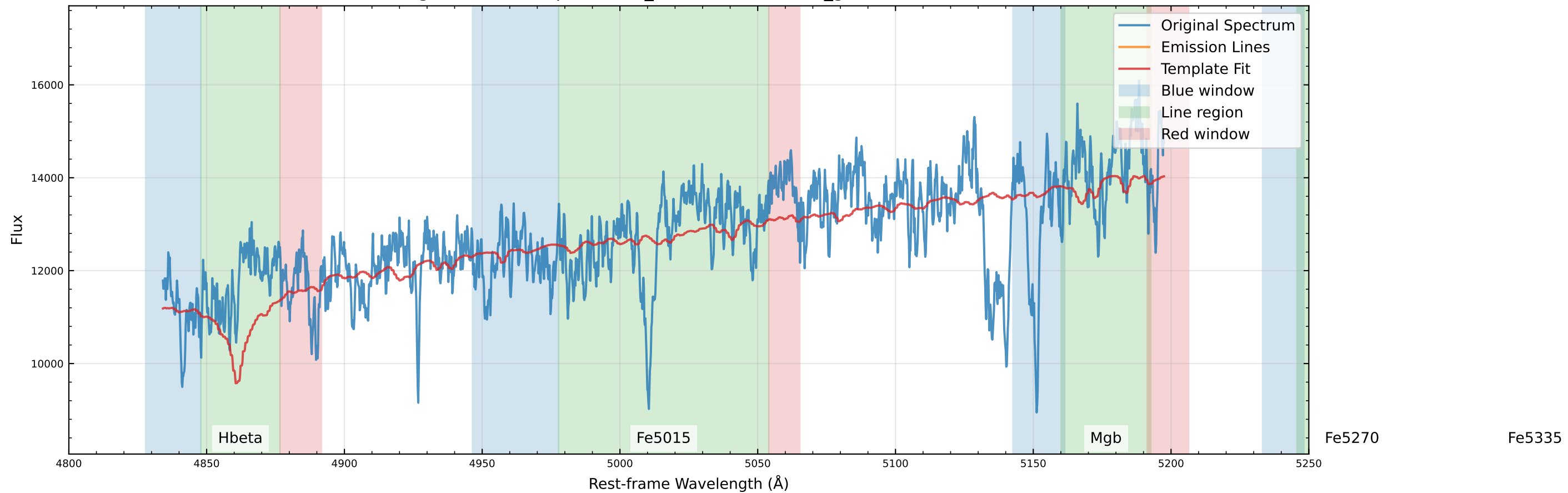
Original Data Comparison (v_star=445.9 km/s, v_gas=459.7 km/s)
