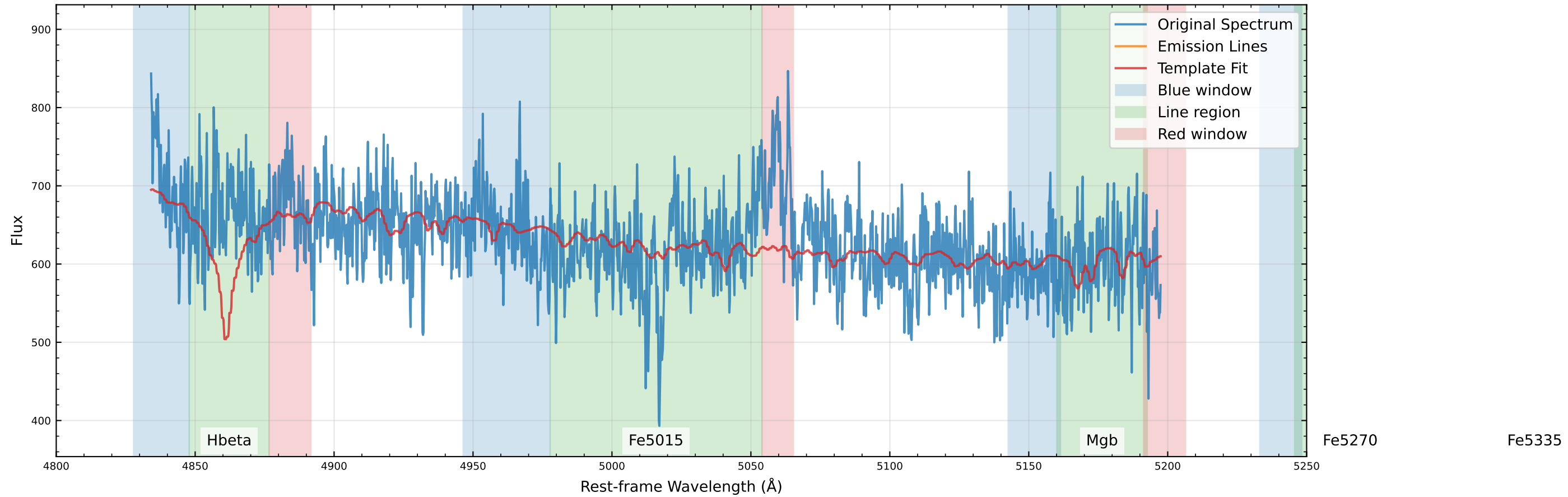
Original Data Comparison (v_star=-387.9 km/s, v_gas=-87.9 km/s)
