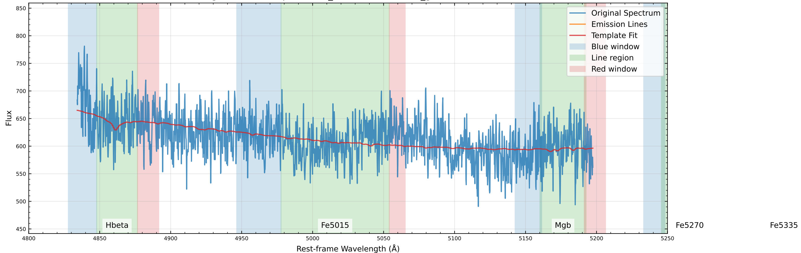
Original Data Comparison (v_star=102.8 km/s, v_gas=82.3 km/s)
