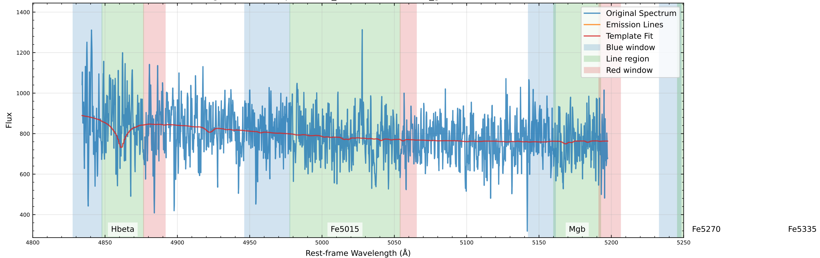
Original Data Comparison (v_star=-100.1 km/s, v_gas=-400.1 km/s)
