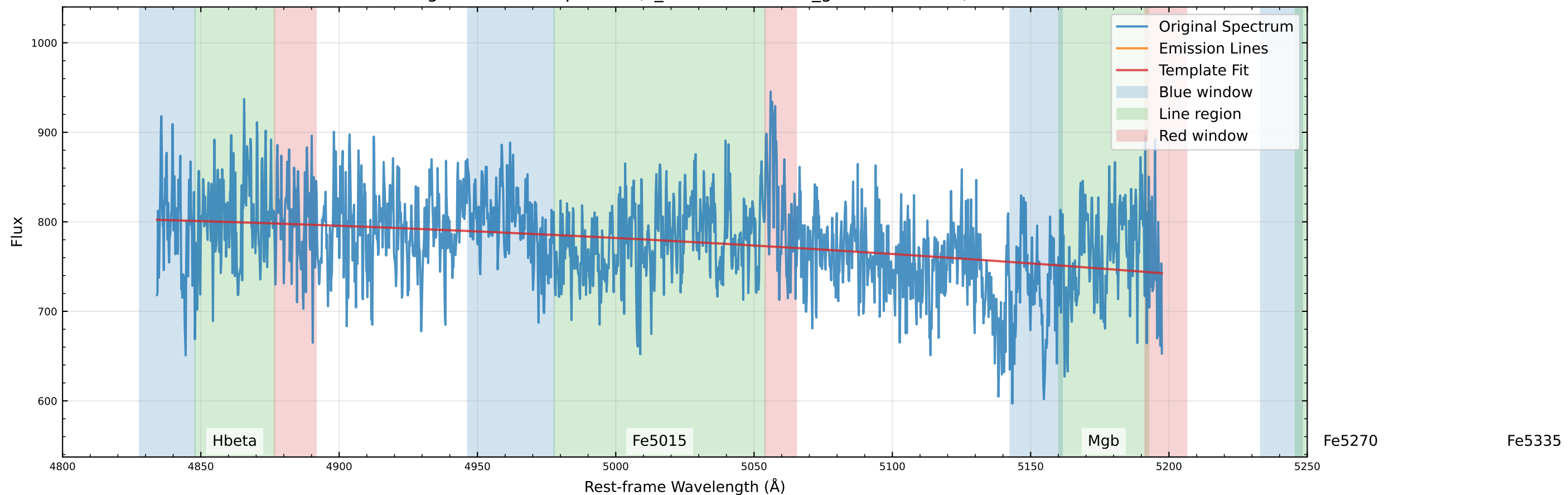
Original Data Comparison (v_star=0.0 km/s, v_gas=-25.2 km/s)
