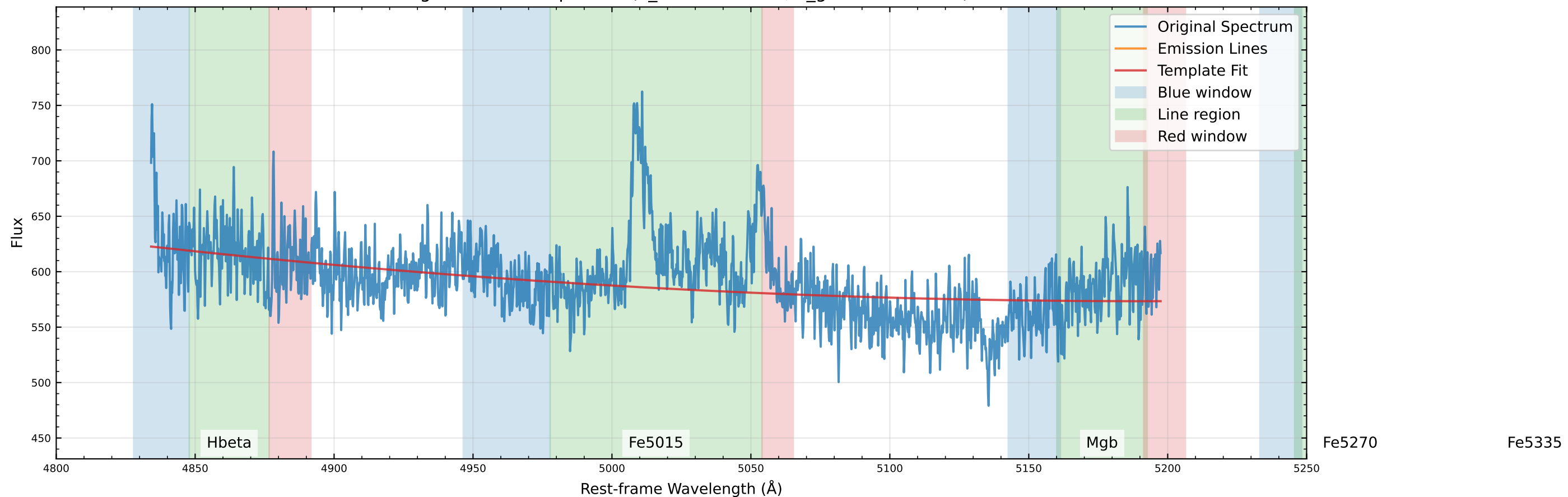
Original Data Comparison (v_star=0.0 km/s, v_gas=196.5 km/s)
