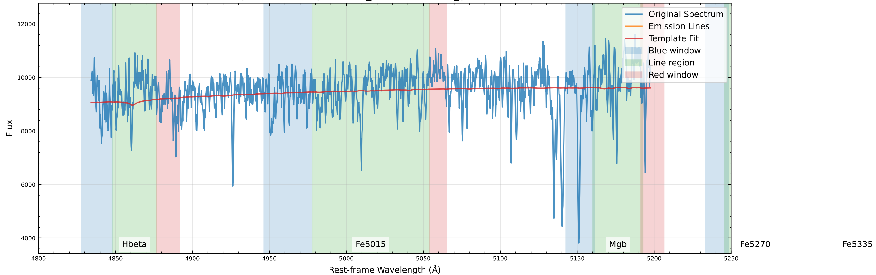
Original Data Comparison (v_star=9.0 km/s, v_gas=309.0 km/s)
