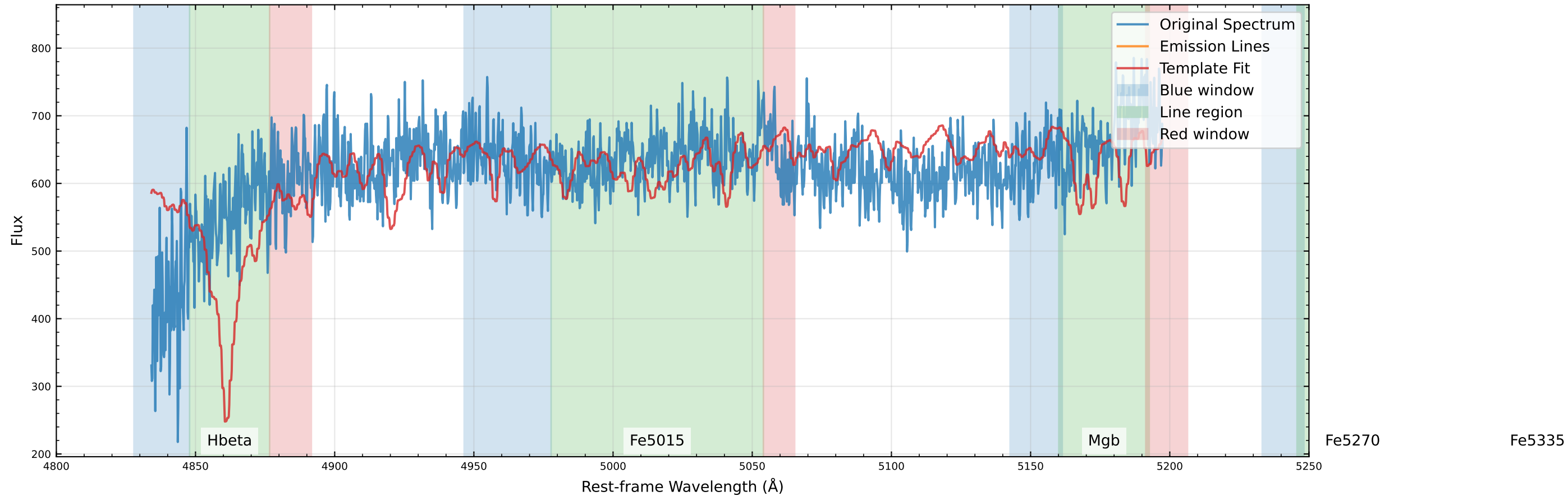
Original Data Comparison (v_star=-293.0 km/s, v_gas=-429.3 km/s)
