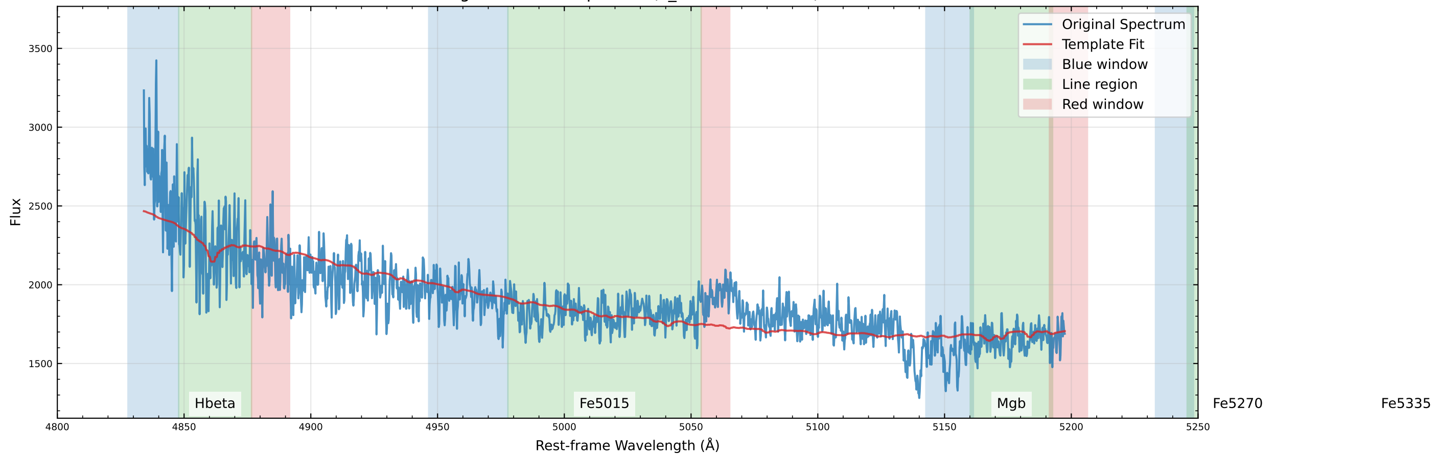
Original Data Comparison (v_star=132.1 km/s)
