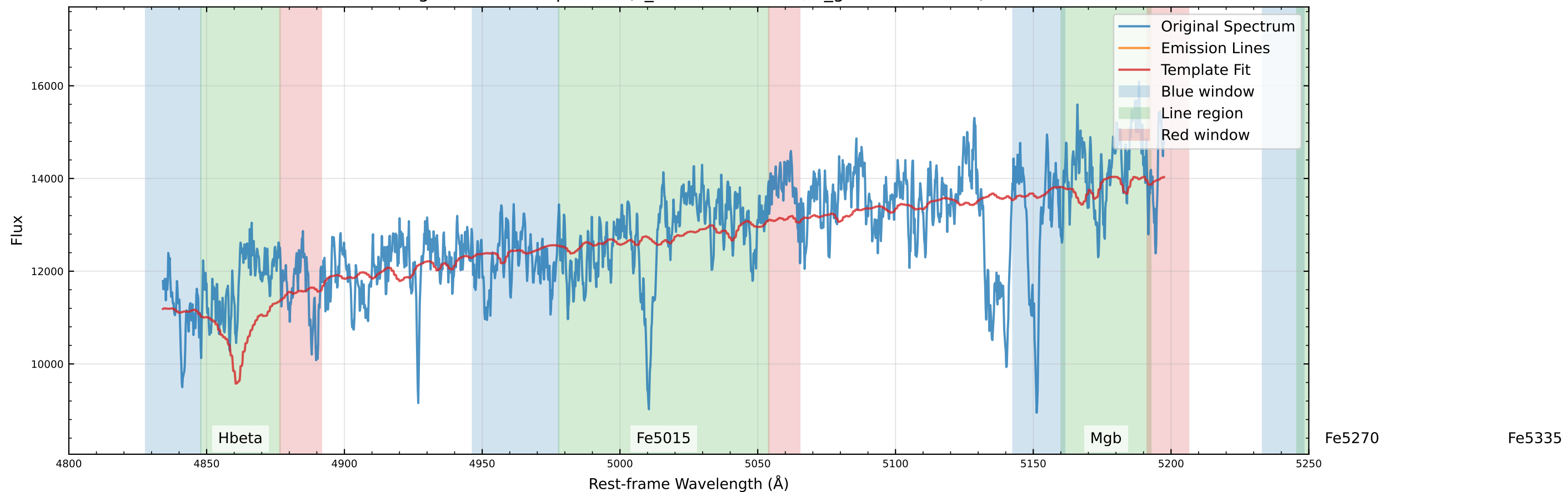
Original Data Comparison ( v_{\text{star}}=445.9 km/s, v_{\text{gas}}=459.7 km/s)
