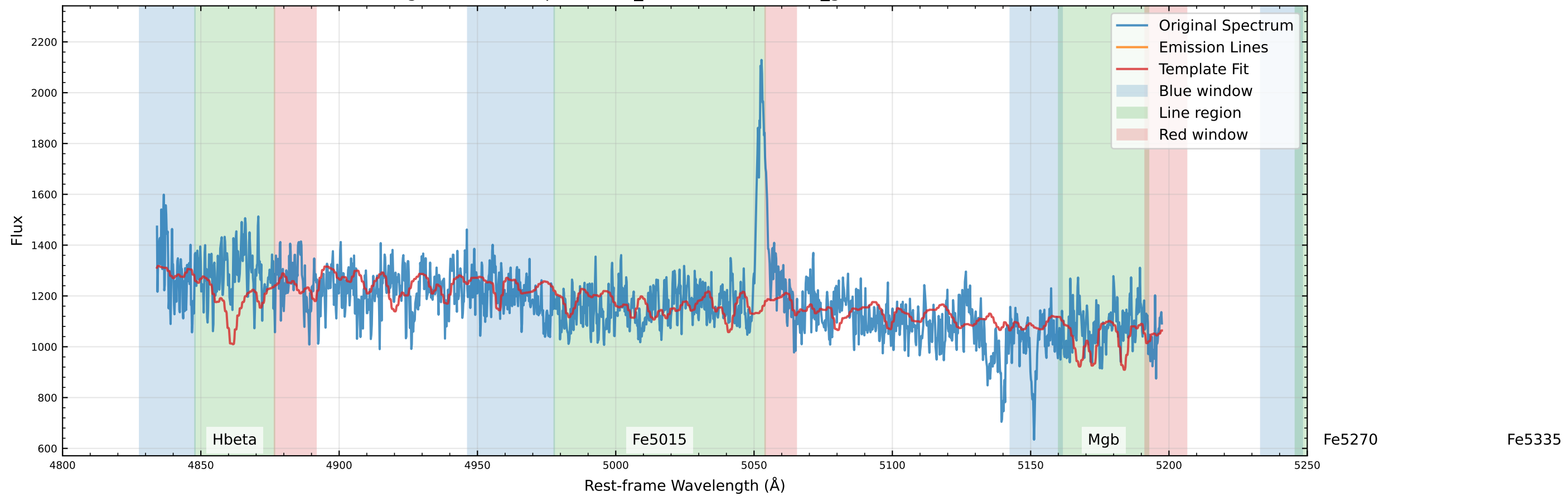
Original Data Comparison (v_star=-558.1 km/s, v_gas=-258.1 km/s)
