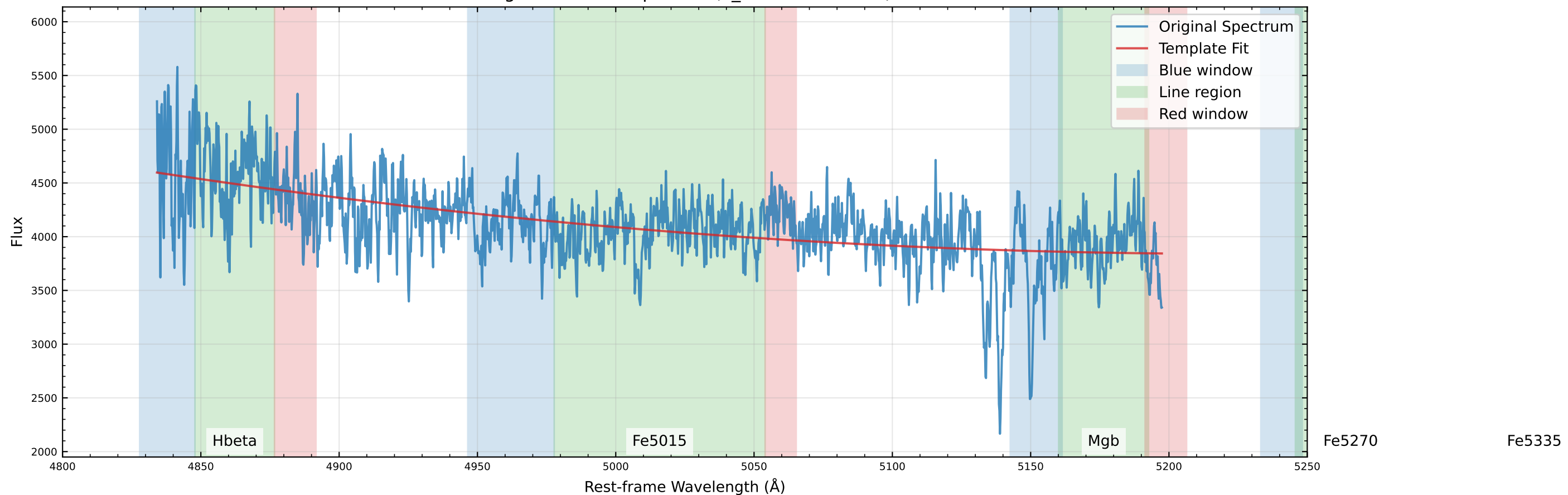
Original Data Comparison (v_star=-12.1 km/s)
